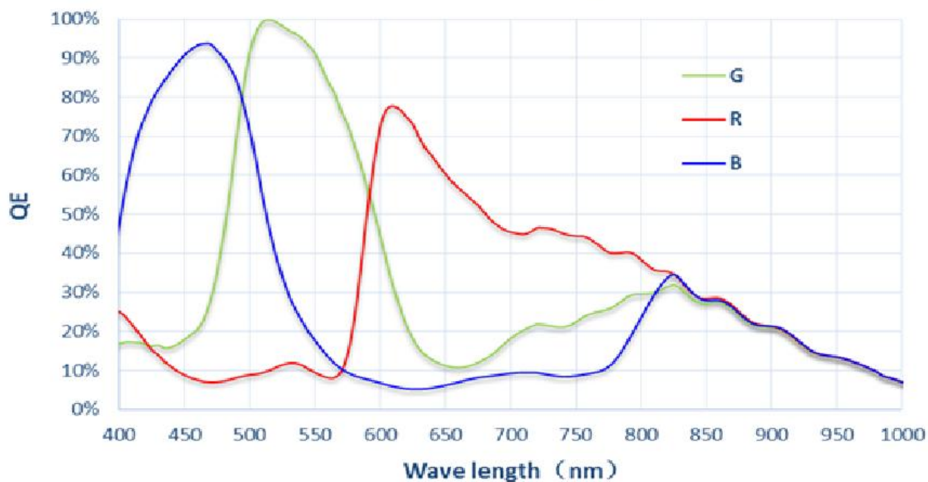
SC130GS Relative QE
